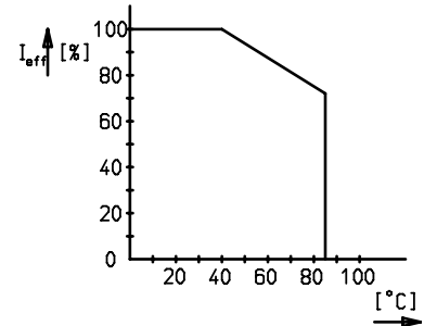
load diagram
